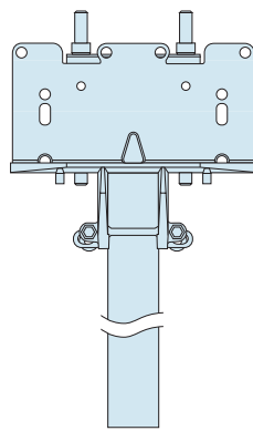
Bracket assembly
