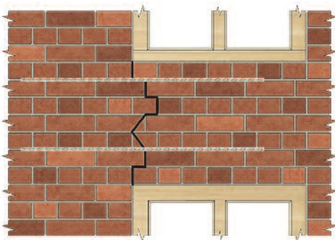
Crack stitching
