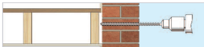
1. Mark the position of the joist centre on the external wall and then drill a clearance hole (normally 16mm) through the wall. Clean out the hole
