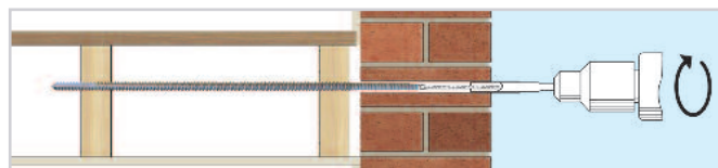
2. Fit the BowTie HD Support Tool to an SDS rotary hammer drill, insert the BowTie HD and drive it (off hammer) into, and through, the first and second joists
