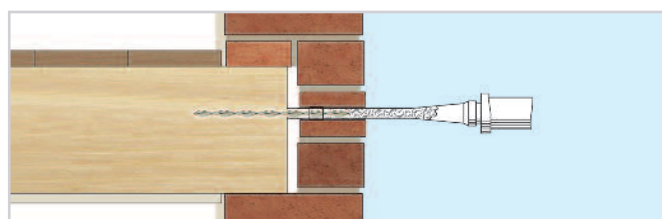
4. Inject EpoxyPlus EX resin to fill the hole and bond the BowTie to the masonry and then make good
