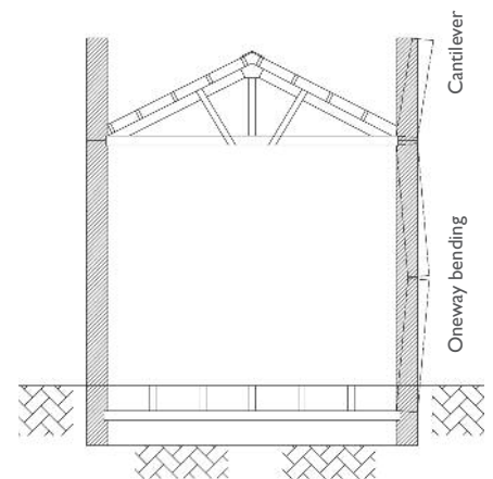
Figure 2 Deflected shapes of a properly secured URM wall when subjected to out-of-plane seismic forces
