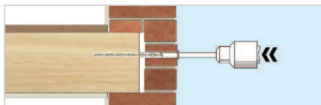
2. Fit the BowTie Support Tool to an SDS rotary hammer drill, insert the BowTie and drive it into joist end to the required depth – at least 75mm (or through the second joist if parallel)
