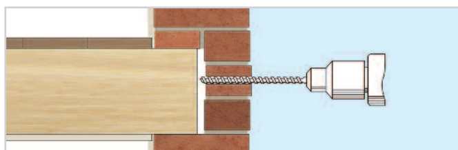
1. Mark the position of the joist centre on the external wall and then drill a clearance hole (normally 12mm) through the wall (and first joist if parallel to the wall). Clean out the hole
