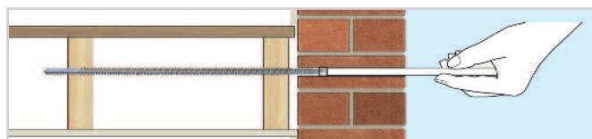
4. Fit the plastic sleeve over the BowTie HD and use the support tool to push it to the back of the hole in the wall (outer leaf in a cavity wall)
