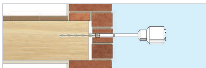
3. Fit the plastic sleeve over the BowTie and use the support tool to push it to the back of the hole in the masonry (in the outer leaf in a cavity wall)
