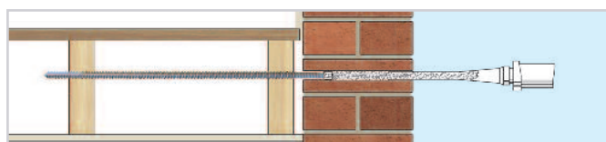
5. Inject EpoxyPlus EX resin to fill the hole and bond the BowTie HD to the masonry, allow the resin to gel and then make good
